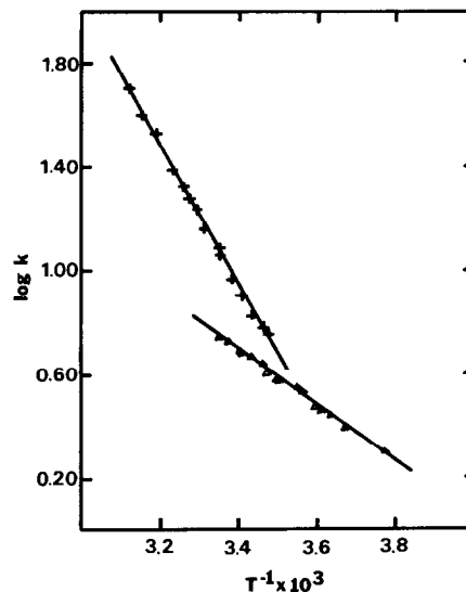
Figure 4. Arrhenius least-squares plots for acetylacetonate methyl group (+) and isopropyl methyl group exchange (Δ) in the \text{Ti}(\text{acac})_2(2\text{-}^i\text{PrC}_6\text{H}_4\text{O})_2 complex in dichloromethane solution.
