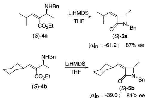
Scheme 2. Synthesis of Alkylidene- \beta -lactams 5a–b
