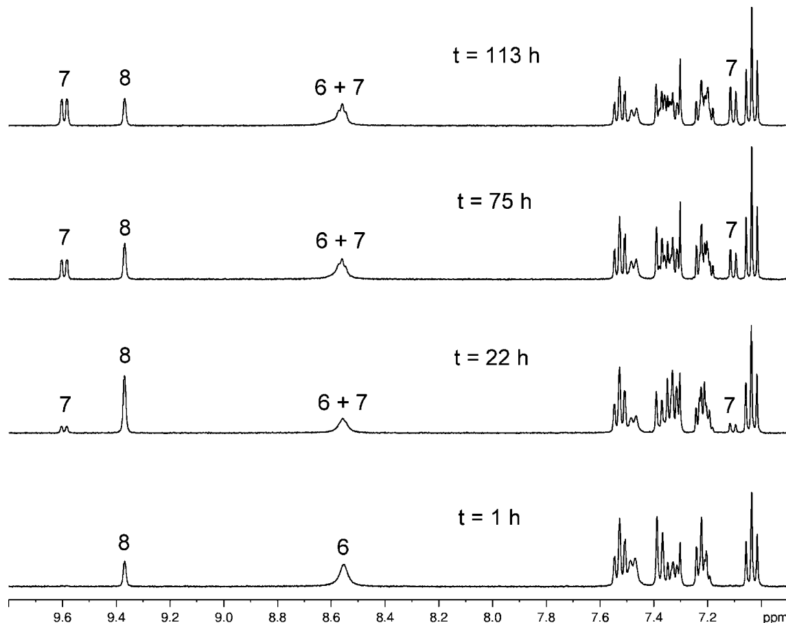
Figure 4. NMR spectra of a representative tautomerization reaction, showing selected diagnostic resonances of compounds 6 , 7 , and 8 .
