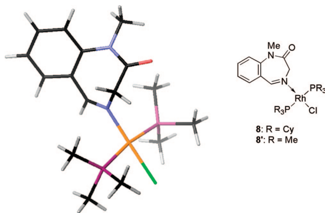
Figure 3. DFT geometry-optimized structure for 8' .
