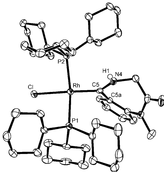
Figure 5. ORTEP drawing of 7 . 19 Thermal ellipsoids are drawn at the 50% probability level. Two molecules of THF have been deleted for clarity. Hydrogens other than H(1) have been omitted for clarity. Selected bond distances (Å) and angles (deg): Rh–C(5), 1.914(3); C(5)–N(4), 1.330(4); C(5)–C(5a), 1.506(4); N(1)–H(1), 0.79(3); Rh–P(1), 2.345(1); Rh–P(2), 2.333(8); Rh–Cl, 2.4456(8); N(4)–C(5)–C(5a), 113.1(3); Rh–C(5)–N(4), 129.4(2); Rh–C(5)–C(5a), 117.4(2); P(1)–Rh–P(2), 159.05(3); Cl–Rh–C(5), 166.15(9); Cl–Rh–P(1), 88.67(3); Cl–Rh–P(2), 87.66(3); P(1)–Rh–C(5), 94.10(9); P(2)–Rh–C(5), 94.37(9).
