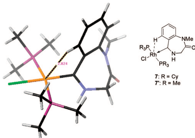
Figure 2. DFT geometry-optimized structure of 7' illustrating the preagostic interaction between the C6–H bond and the rhodium center.
