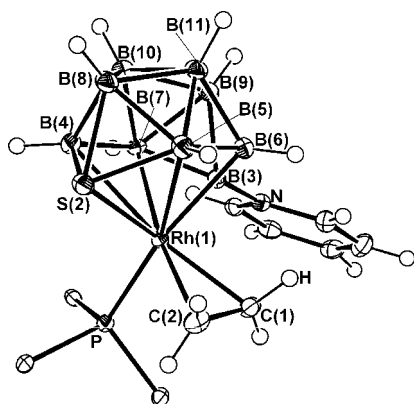
Figure 3. Molecular structure of [1,1-(\text{PPh}_3)(\eta^2\text{-C}_2\text{H}_4)\text{-}3\text{-(NC}_5\text{H}_5)\text{-closo-}1,2\text{-RhSB}_9\text{H}_8] ( 3 ).
