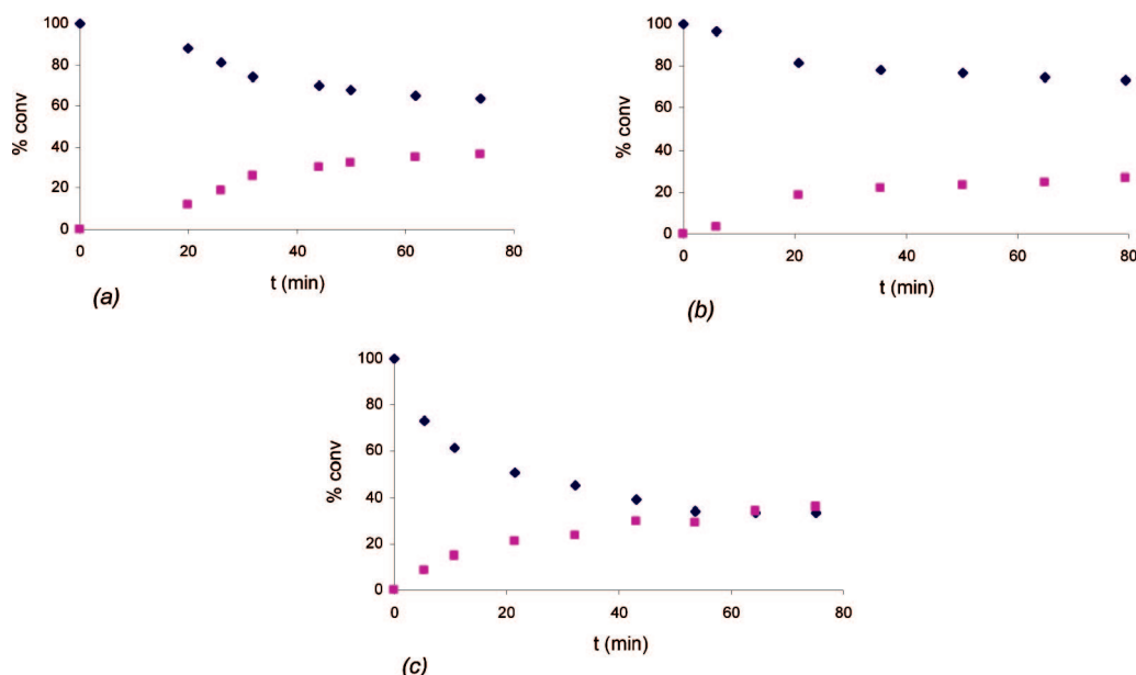
Figure 5. Plots of reaction time vs conversion based on ^1\text{H} NMR signal intensities for reaction of 3 and 5 with \text{H}_2(\text{g}) : (a) in \text{CD}_2\text{Cl}_2 with a 1:1 ratio of 3 to free \text{PPh}_3 , (b) 5 in \text{CD}_2\text{Cl}_2 , and (c) 3 in (\text{CD}_3)_2\text{CO} ( closo compounds 3 and 5 , dark blue diamonds; nido -rhodathiaborane 2 , magenta squares).
