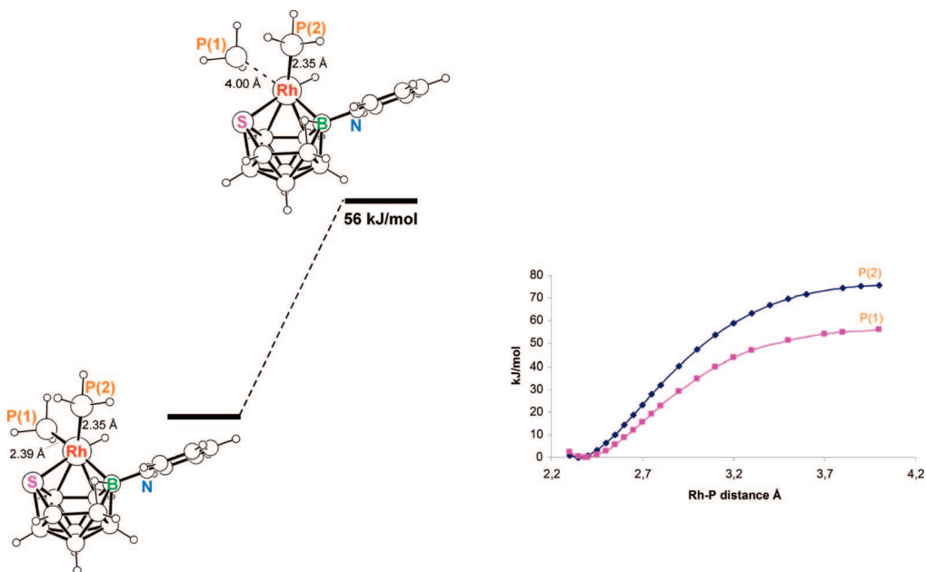
Figure 2. DFT-calculated energies (kJ/mol) computed at the B3LYP/6-31G*/LANL2DZ level for elongation of the \text{PH}_3 ligands in the model [8,8,8-( \text{PH}_3 ) _2 H-9-( \text{NC}_5\text{H}_5 )-nido-8,7-RhSB _9 H _9 ] ( 2a ).
