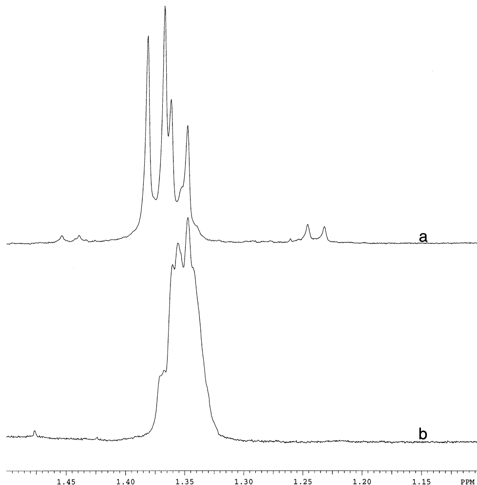
Fig. 2. ^1\text{H} -NMR-spectrum (1:1 (\text{CF}_3)_2\text{CDOD}-\text{CDCl}_3 ; 500 MHz) of poly(styrene- alt -CO) prepared with 1 (a) and 2 (b).
