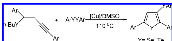
Scheme 1. General Scheme
