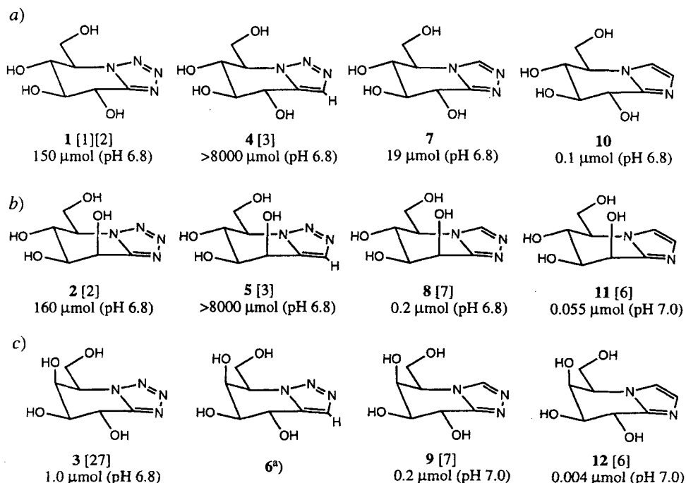
Fig. 2. K_i Values of gluco-, manno-, and galacto-configured tetrahydropyridoazoles against a) sweet-almonds \beta -glucosidases, b) snail- \beta -mannosidase, and c) E. coli \beta -galactosidase
