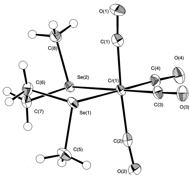
Fig. 1. Structure of [\text{Cr}(\text{CO})_4\{\text{MeSe}(\text{CH}_2)_2\text{SeMe}\}] with atom numbering scheme. Ellipsoids are drawn at the 40% probability level.
