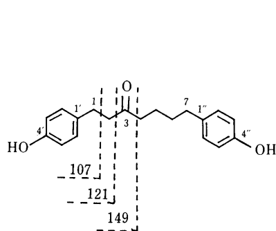
acerogenin G ( 3 )
