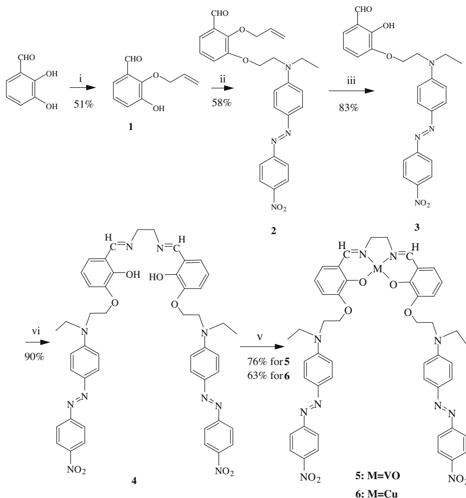
Scheme 1. Reagent and conditions: (i) allyl bromide/NaH; (ii) p -[HOCH 2 CH 2 N(C 2 H 5 )] 2 C 6 H 4 N 2 C 6 H 4 -( p -NO 2 ), DR1 , DEAD/PPh 3 ; (iii) DMF–H 2 O/Pd–C; (iv) H 2 NCH 2 CH 2 NH 2 ; (v) Cu(OAc) 2 or VO(acac) 2 /EtOH.
