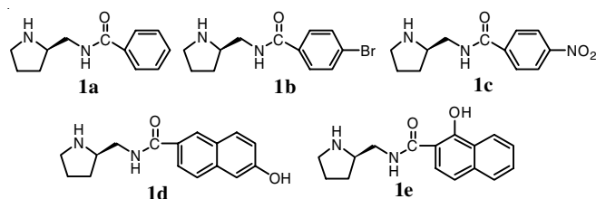
Fig. 1. Secondary amine-amide catalysts
