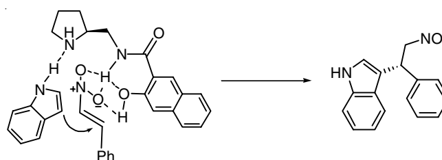
Fig. 2. Possible mechanism of catalyst 1e
