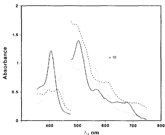
Fig. 3. Spectroelectrochemistry of 0.2 mM [\text{Fe}(\text{TPP})]_2(\text{SO}_4) in methylene chloride in OTTLE cell. Solid line: 0 V vs. SRE; dotted line: -0.9 V vs. SRE; dashed line: -1.8 V vs. SRE. 476-750 nm region was multiplied by a factor of 10.
