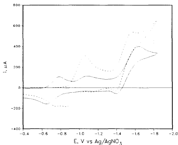
Fig. 4. Cyclic voltammetry of [\text{Fe}(\text{TPP})]_2(\text{SO}_4) in the presence and absence of sulfate in methylene chloride. Solid line: 0 mM sulfate; dotted line: 1 mM sulfate; dashed line: 10 mM sulfate. Concentration of [\text{Fe}(\text{TPP})]_2(\text{SO}_4) : 0.5 mM; platinum working electrode; scan rate = 100 mV/s.
