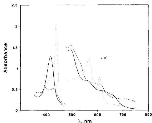
Fig. 5. Spectroelectrochemistry of 0.2 mM [\text{Fe}(\text{TPP})]_2(\text{SO}_4) in methylene chloride in the presence of 5 mM sulfate in an OTTLE cell. Solid line: -0.4 V vs. SRE; dotted line: -1.0 V vs. SRE; dashed line: -1.8 V vs. SRE. 476-750 nm region was multiplied by a factor of 10.
