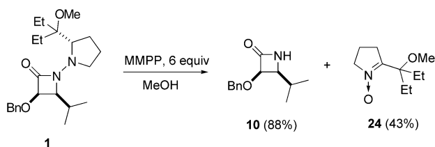
Scheme 6. Cleavage of proline derivative 1 by excess of MMPP.
