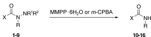
Scheme 4. Deamination of hydrazides by peracids.
