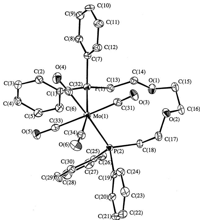
Fig. 1. View of the structure of cis -[Mo(CO) _4 (L ^1 )] with numbering scheme adopted. Ellipsoids are drawn at 40% probability. H atoms are omitted for clarity.
