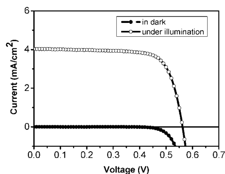
Figure 5. Current versus voltage in the constructed cell. V_{\text{oc}} = 562\text{ mV} , J_{\text{sc}} = 4.03\text{ mA/cm}^2 , FF = 0.735, \eta = 1.66\% . Cell's active surface area was 0.159\text{ cm}^2 , and the illumination intensity was 100\text{ mW/cm}^2 at 1.5 AM conditions.
