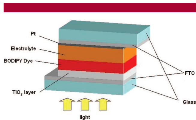
Figure 2. Schematic drawing of a dye-sensitized solar cell: the BODIPY dye is placed under the F-doped \text{SnO}_2 layer and adsorbed to nanocrystalline \text{TiO}_2 .
