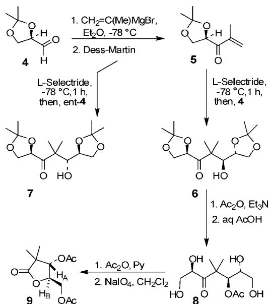
Scheme 1. Asymmetric Reductive Aldol Reaction of Chiral Enone with Chiral Aldehydes
