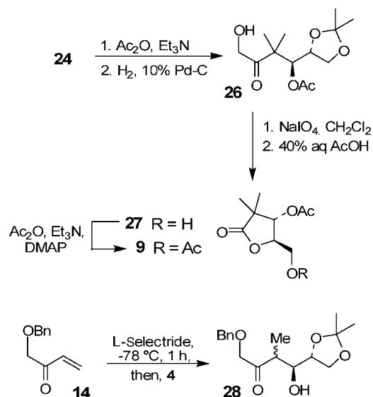
Scheme 3. Synthesis of 9 and Aldol Reaction of 14
