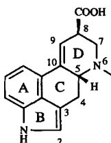
II Lysergic acid
