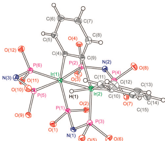
Figure 2. Solid state structure of \text{Ir}_2^{\text{I,III}}(\text{tfpma})_3(\mu\text{-C}_6\text{H}_4)(\text{C}_6\text{H}_5)\text{H} ( 3 ). Ellipsoids are drawn at the 50% probability level with -\text{NMe} and -\text{CH}_2\text{CF}_3 groups removed for clarity.
