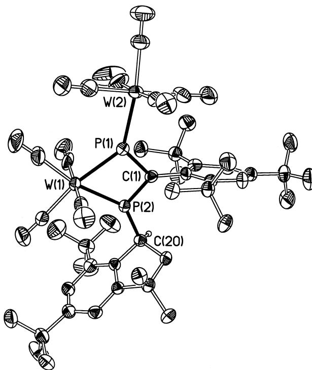
Fig. 2. Molecular structure of 3 : Selected bond lengths (Å) and angles ( ^\circ ): P(1)–W(1) 2.464(2), P(1)–W(2) 2.443(2), P(1)–C(1) 1.803(6), P(2)–W(1) 2.411(2), P(2)–C(1) 1.716(6), P(2)–C(20) 1.860(6), P(1)–C(1)–P(2) 96.1(3), W(1)–P(1)–C(1) 97.2(2), W(1)–P(2)–C(1) 101.7(2), P(1)–W(1)–P(2) 64.9(3).
