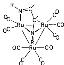
Fig. 3. One of the expected structures for \text{Ru}_3(\text{CO})_9(\text{R-DAB}) . For the actual structure see Table II.
