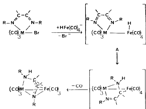
Scheme 3. Possible reaction pathway for the formation of \text{FeM}(\text{CO})_6(\text{R-AAA}) ( \text{M} = \text{Mn}, \text{Re} ).
