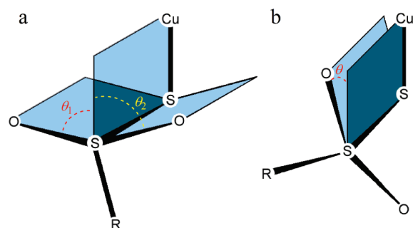
Figure 7. Torsion angles describing the orientation of the SO 2 R group relative to the Cu–S bond: (a) type I (−50° < θ 1 < −70°, 50° < θ 2 < 70°) and (b) type II (−10° < θ < 10°).
