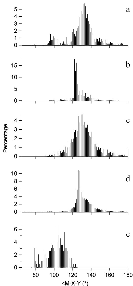
Figure 9. Distribution of M–X–Y angles for oxoanion coordination complexes (number of structures) of (a) sulfate (999); (b) arsenate (495); (c) perchlorate (1223); (d) phosphate (6502); and (e) \text{SXO}_3^{n-} (198) ( X = \text{S}, \text{P}, \text{Si} , and esters thereof).
