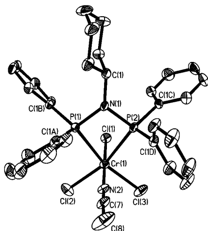
Figure 1. ORTEP diagram of complex 2 ( \text{R} = \text{Cy} ) with thermal ellipsoids at the 40% probability level. Hydrogen atoms have been omitted for clarity.
