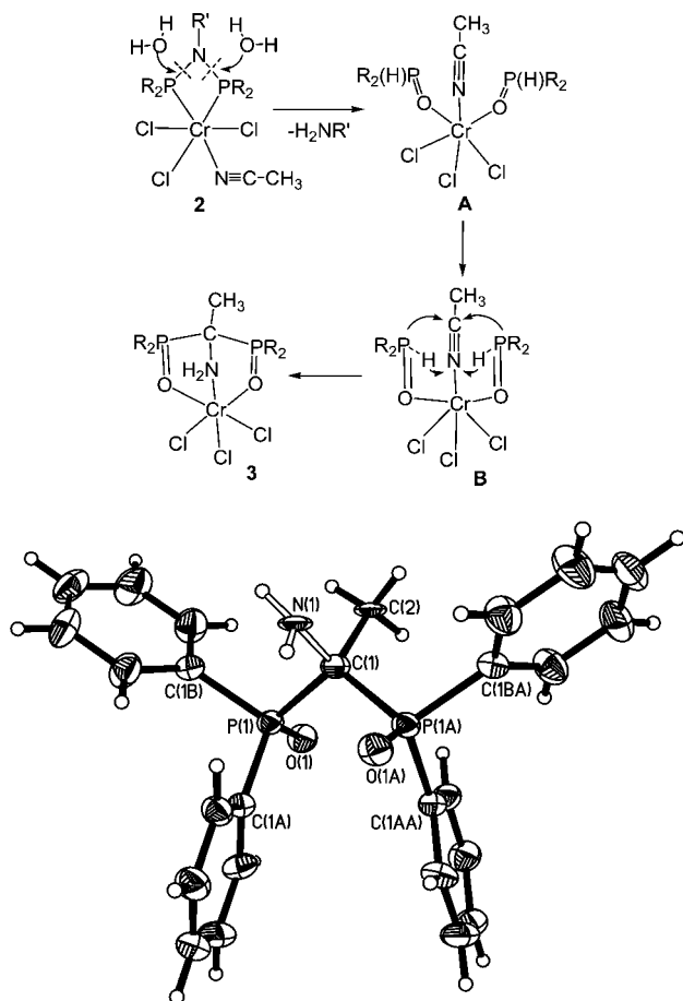
Figure 3. ORTEP diagram of complex 4 with thermal ellipsoids at the 40% probability level. Selected bond lengths [Å] and bond angles [deg]: P(1)–O(1) 1.490(3), P(1)–C(1) 1.879(3), C(1)–N(1) 1.476(11), O(1)–P(1)–C(1) 112.47(12), N(1)–C(1)–C(2) 107.4(5), N(1)–C(1)–P(1) 112.6(4), C(2)–C(1)–P(1) 107.6(4).
