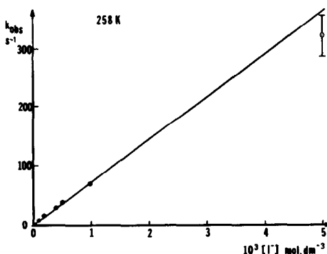
Fig. 3. Plot of first order rate constant ( k_{\text{obs}} ) versus [\text{CTA}^+\text{I}^-] in dichloromethane at 258 K at constant \text{D}^+\text{SbF}_6^- concentration.
