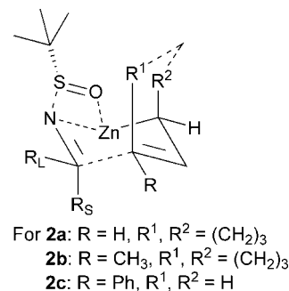
Figure 3. Possible transition state (TS-1).
