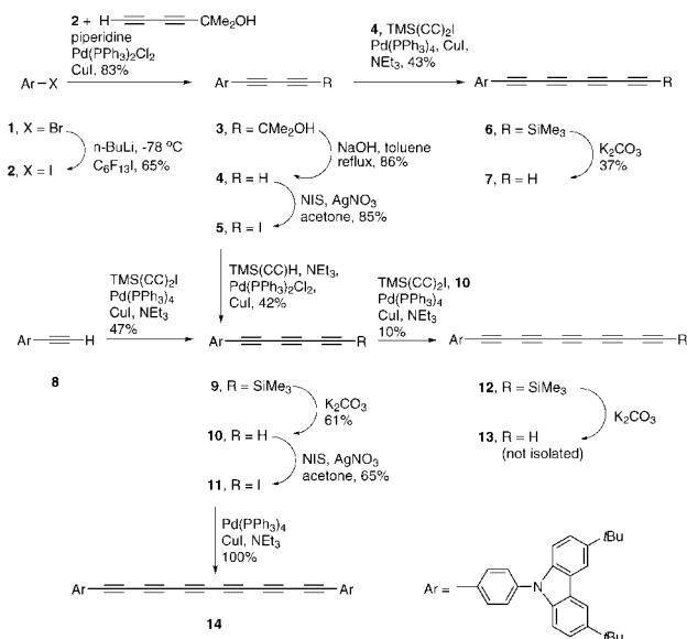
Scheme 1. Synthesis of the Terminal Aryl Oligoynes
