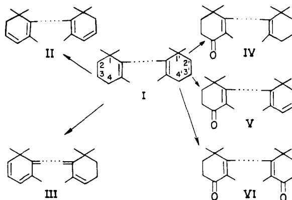
Chart 1.—Conversion of \beta -carotene (I) by N-bromosuccinimide in chloroform in the presence of 1% ethanol.
