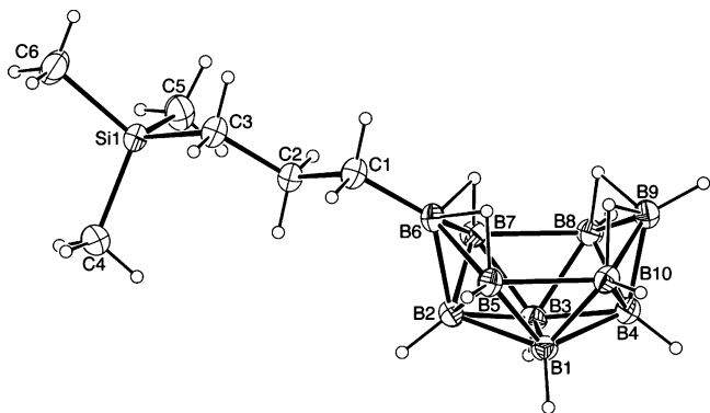
Figure 3. ORTEP representation of the structure of 6-[( CH_3 ) _3Si(CH_2)_3 ]- B_{10}H_{13} ( 2 ). Selected bond lengths (Å) and bond angles (deg): C6–Si, 1.860(2); C4–Si, 1.862(2); C5–Si, 1.864(2); Si–C3, 1.870(2); C1–B6, 1.574(3); B6–B5, 1.800(3); B5–B10, 1.983(3); B6–B7, 1.805(3); B7–B8, 1.977(3); B10–B9, 1.790(3); C4–Si–C5, 108.78(13); C6–Si–C3, 110.02(12); C5–Si–C3, 109.09(10); C2–C1–B6, 114.0(2); C1–B6–B2, 132.1(2); C1–B6–B7, 127.6(2); C1–B6–B5, 127.5(2); B6–B7–B8, 118.25(14); B6–B5–B10, 117.41(14).
