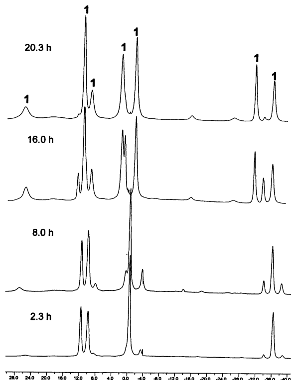
Figure 2. Reaction progression for the reaction of B_{10}H_{14} with 1-octene in bmpyBF_4 /toluene, as measured by the ^{11}B\{^1H\} NMR spectra of the toluene layer versus time. 1 = (6-octyl- B_{10}H_{13} ) resonances.
