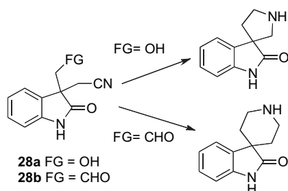
Fig. 3. 3-Functionalized-3-cyanomethyl-oxindoles as precursor of spiropyrrolidinyl- and spiropiperidinyloxindoles.
