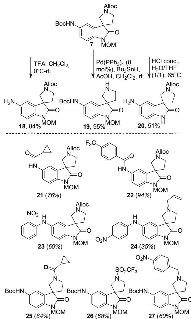
Fig. 2. Functionalized spiropyrrolidinyloxindoles.
