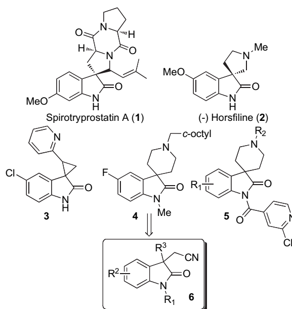
Fig. 1. Natural and synthetic 3,3'-spirooxindoles.
