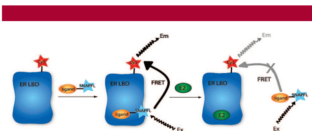
Figure 2. Schematic of SNAPFL-Cy5 FRET. Cy5-labeled ER (left) binds cyclofenil-SNAPFL ( 2 ) and FRET is observed (middle). When excess estradiol out-competes the ligand-fluorophore (right), FRET signal is decreased.
