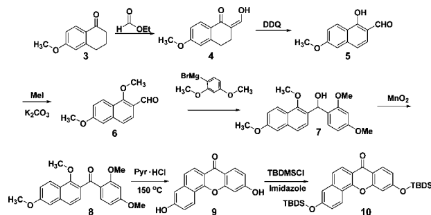
Scheme 1. Synthetic Scheme To Prepare for Benz[ c ]xanthene-7-one ( 10 )
