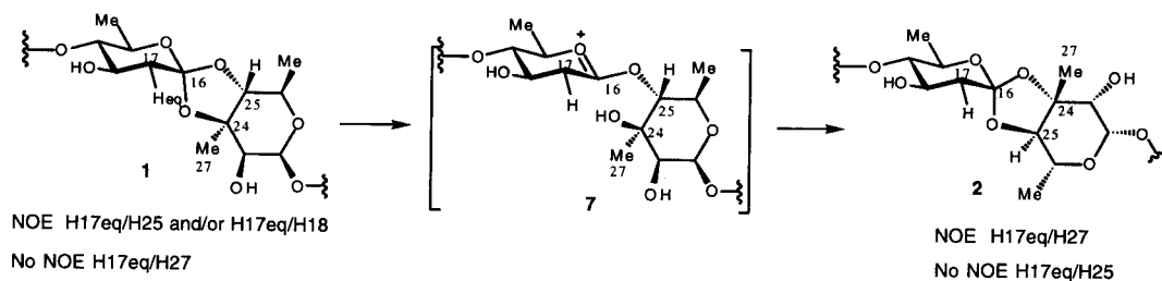
Scheme 2 Observed NOE differences in 1-2
