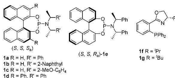
Figure 1. Chiral ligands 1a–g .
