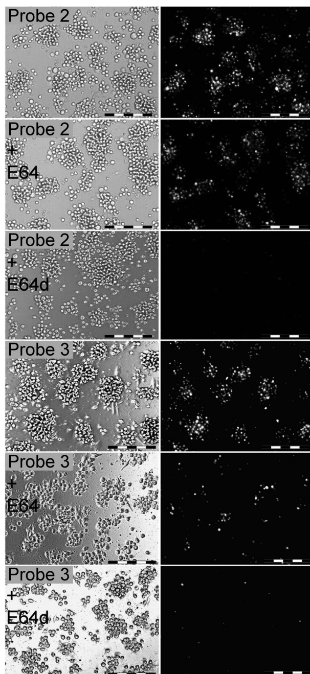
Figure 2. Bright-field (left) and NIR fluorescence (right, ( \lambda_{ex}=635 –675 nm, \lambda_{em}=696 –736 nm) images of PMA-differentiated THP-1 cells incubated with probe 2 ( t=1 h) or lipidated probe 3 ( t=4 h). Longer incubation time for probe 3 was required to overcome the effect of self-quenching. Cells were incubated with the cell-impermeant cathepsin inhibitor E-64 or its cell-permeant form E-64d for 1 h prior to addition of the probe. Scale bar = 200 \mu m. PMA = phorbol ester.
