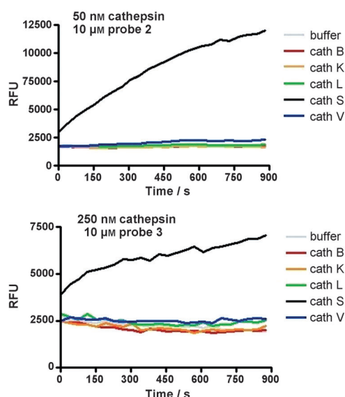
Figure 1. Cleavage of cathepsin S reporters in vitro. Change in emission intensity at \lambda_{em}=695 nm ( \lambda_{ex}=670 nm) of 2 (a) and lipidated probe 3 (b) after addition of various cathepsins. RFU = relative fluorescence units.
