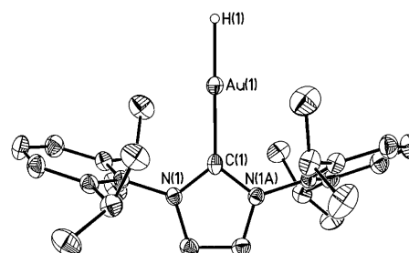
Figure 1. Solid-state structure of 2 (C 5 H 12 ); thermal ellipsoids are set at the 50% probability level. For clarity, hydrogen atoms (except for that bound to the gold atom) and solvent molecule are omitted. Selected bond lengths [Å] and angles [°]: Au(1)–C(1) 2.045(3), C(1)–N(1) 1.362(3); N(1)–C(1)–Au(1) 127.98(14), N(1)–C(1)–N(1A) 104.0(3). N(1A) is a crystallographic symmetry equivalent of N(1), generated by the operator -x+2, y, -z+1/2 .
