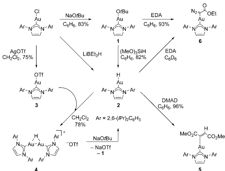
Scheme 1. Preparation and reactions of 2 . OTf = CF 3 SO 3 , DMAD = dimethyl acetylenedicarboxylate, EDA = ethyl diazoacetate.
