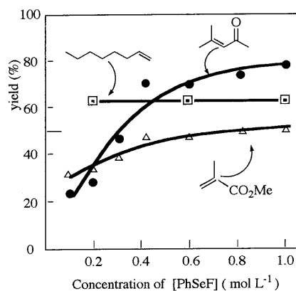
Fig. 1. Effect of the concentration of [PhSeF].
