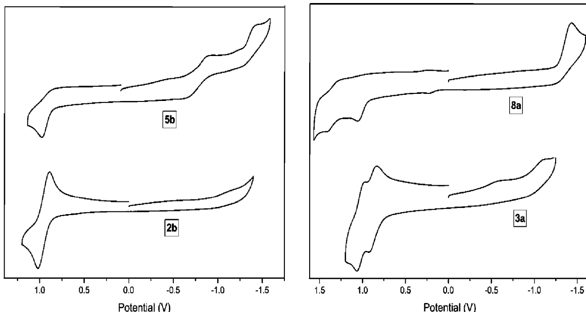
Figure 4. Cyclic voltammograms of (a) monocobaloximes and (b) biphenyl-bridged dicobaloximes in DCM with 0.1 M ( ^t\text{Bu}_4\text{NPF}_6 ) as supporting electrolyte at 0.2 V \text{s}^{-1} at 25 °C.
