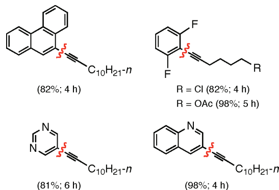
Scheme 3. Additional Couplings Using Ligand 14 in PTS/ \text{H}_2\text{O}
