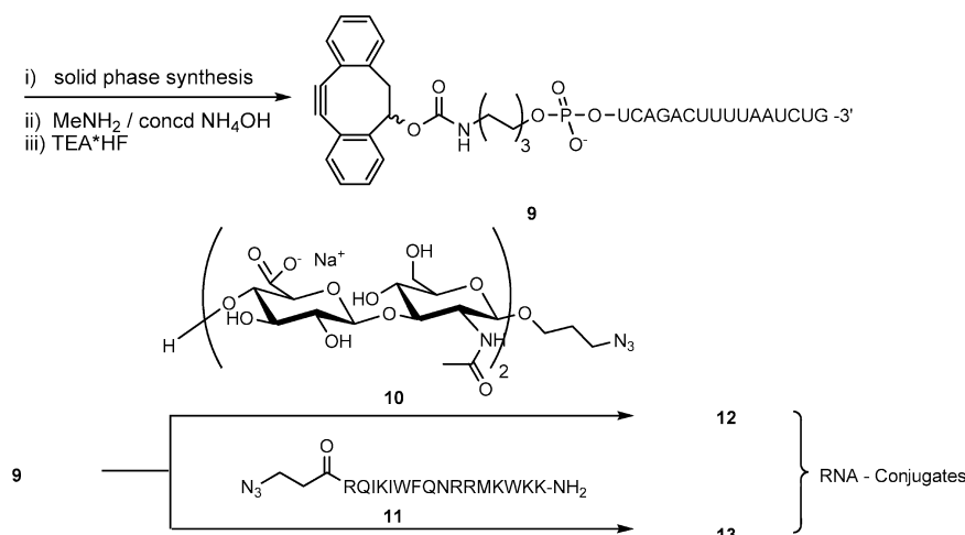
Scheme 3. Synthesis of 5'-Alkyne Functionalized Ribonucleic Acid 16-mer and Its Conjugation to Hyaluronic Acid Tetramer and Penetratin
