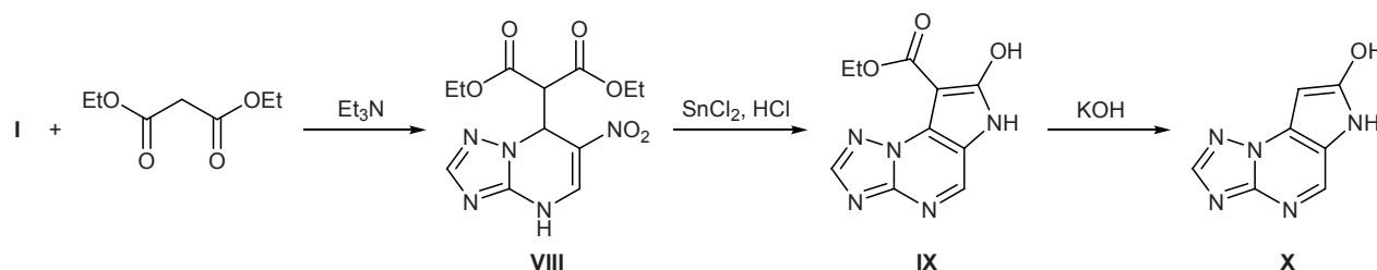
Scheme 4.
