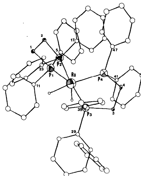
Fig. 1. The molecular structure of \text{H}_2\text{Ru}(\text{Ph}_2\text{PCH}_2\text{CH}_2\text{PPh}_2)_2 \cdot \text{C}_6\text{H}_6 , as viewed along the b axis. For the sake of clarity the first carbon atom of each phenyl ring has been labelled with a number. The solvated benzene is shown in the lower part of the figure.
