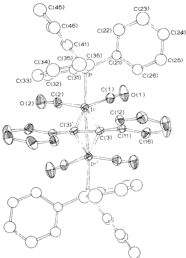
Fig. 2. ORTEP view of the \{[\text{Ir}(\text{CO})_2\text{PPh}_3]_2(\text{CPh})_2\} molecule, with the hydrogen atoms omitted for clarity. Thermal ellipsoids are drawn at 30% probability
