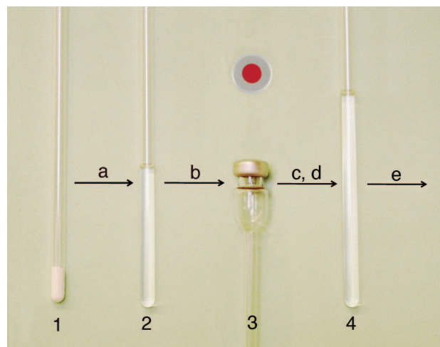
Figure 1. Graphical representation of the water determination experiment. From left to right: (1) \text{TBAF}/\text{PhI}(\text{OAc})_2/\text{TBABF}_4 mixture in a reaction tube; (2) assay mixture dissolved in \text{CD}_3\text{CN} ; (3) side (bottom) and top (top) views of a customized 5 mm NMR tube featuring a fused crimp cap and septum seal; (4) tube containing solid reagents ( \text{TBAF} , \text{TBABF}_4 , \text{PhI}(\text{OAc})_2 ), \text{CD}_3\text{CN} and sample after the addition of the solvent being tested. The process arrows indicate (a) addition of \text{CD}_3\text{CN} , (b) installation of the cap, (c) collection of the background ^{19}\text{F} NMR spectrum, (d) injection of the solvent being tested, and (e) collection of the final ^{19}\text{F} NMR spectrum.
