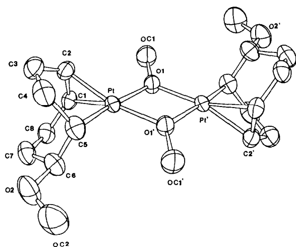
Fig. 1. ORTEP diagram of [\text{Pt}_2(\mu\text{-OCH}_3)_2(\text{C}_8\text{H}_{12}\text{OCH}_3)_2] . Principal bond lengths (Å): \text{Pt}-\text{C}_1 = 2.093(5) , \text{Pt}-\text{C}_2 = 2.098(6) , \text{Pt}-\text{C}_5 = 2.028(6) , \text{Pt}-\text{O}_1 = 2.034(3) , \text{Pt}-\text{O}_1' = 2.153(3) , and bond angles ( ^\circ ): \text{C}_1-\text{Pt}-\text{C}_2 = 39.6(2) , \text{C}_1-\text{Pt}-\text{O}_1 = 95.2(2) , \text{C}_2-\text{Pt}-\text{C}_5 = 82.5(3) , \text{C}_5-\text{Pt}-\text{O}_1' = 98.1(2) , \text{O}_1-\text{Pt}-\text{O}_1' = 76.2(3) .
