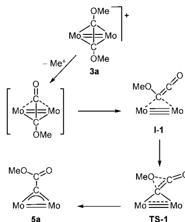
Scheme 1. Proposed Reaction Pathway for the Formation of Compound 5a [ \text{Mo} = \text{MoCp}(\text{CO}) ; the bridging \text{PCy}_2 ligand is omitted for clarity]
