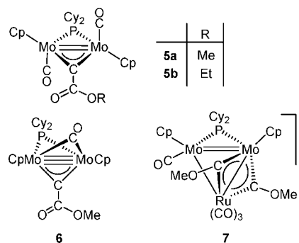
Scheme 1. Proposed Reaction Pathway for the Formation of Compound 5a [ \text{Mo} = \text{MoCp}(\text{CO}) ; the bridging \text{PCy}_2 ligand is omitted for clarity]
