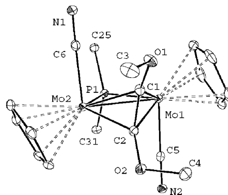
Figure 1. ORTEP diagram (30% probability) of the cation in compound 2 . 2 Cy rings (except the C 1 atoms), t\text{Bu} groups, and H atoms are omitted for clarity.
