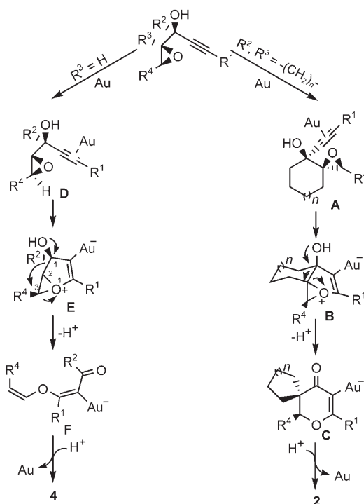
Scheme 3. Proposed mechanism for the gold-catalyzed reactions to form 2 and 4 .
