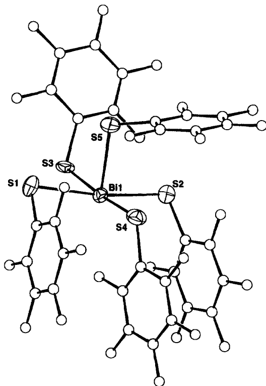
Fig. 1. A view of the structure of the [\text{Bi}(\text{SC}_6\text{F}_5)_5]^{2-} anion in 7 . Thermal ellipsoids are drawn at the 20% level. Selected bond lengths (Å) and angles (°): Bi—S(1) 2.988(9), Bi—S(2) 2.703(9), Bi—S(3) 2.889(9), Bi—S(4) 2.746(10), Bi—S(5) 2.609(10); S(1)—Bi—S(2) 172.0(3), S(1)—Bi—S(3) 92.2(3), S(1)—Bi—S(4) 88.7(3), S(1)—Bi—S(5) 83.7(3), S(2)—Bi—S(3) 89.0(3), S(2)—Bi—S(4) 89.6(3), S(2)—Bi—S(5) 88.6(3), S(3)—Bi—S(4) 175.7(3), S(3)—Bi—S(5) 84.7(3), S(4)—Bi—S(5) 91.2(3).
