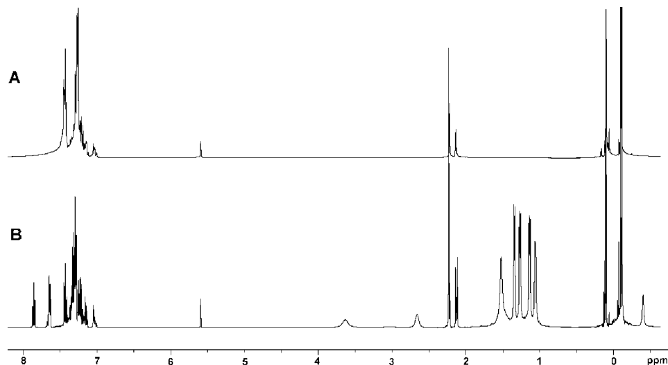
Figure 2. ^1\text{H} NMR spectra (400.13 MHz) of (A) the equimolar reaction of \text{Ph}_3\text{CCl} and \text{LiCH}_2\text{SiMe}_3 and (B) 3b /[ \text{Ph}_3\text{C} ][ \text{B}(\text{C}_6\text{F}_5)_4 ] in chlorobenzene- d_5 at 298 K.
