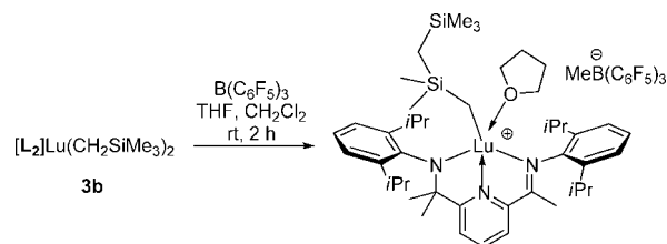
Scheme 2. Cationization of [L 2 ]Lu(CH 2 SiMe 3 ) 2 with B(C 6 F 5 ) 3 (the product was characterized by multinuclear NMR spectroscopy) 13
