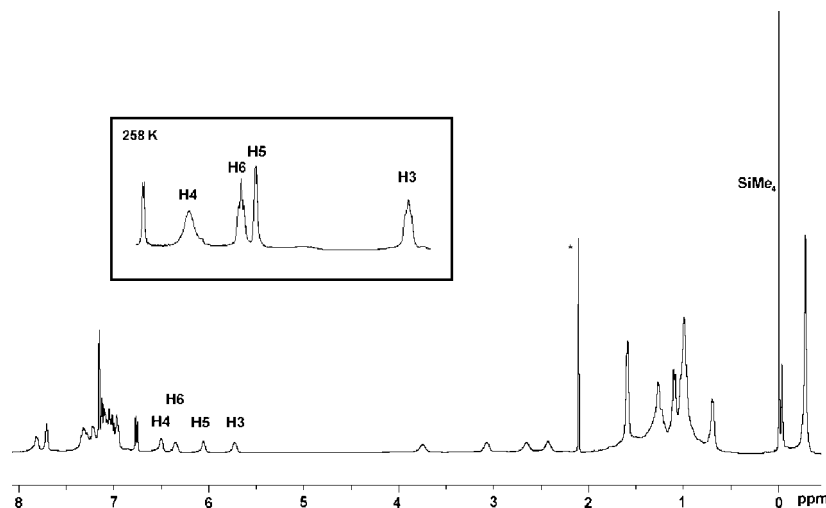
Figure 3. ^1\text{H} NMR spectrum (400.13 MHz) of 3b / N -[tris(pentafluorophenyl)borane]-3 H -indole ( C ) in chlorobenzene- d_8 at 298 K (* = toluene residue).
