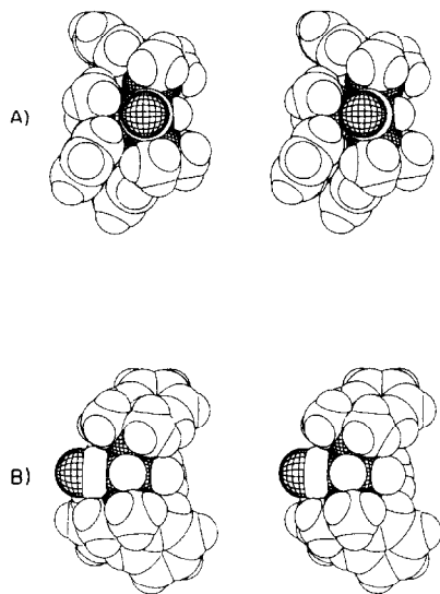
Fig. 4. Stereo space-filling drawings of 1a viewed A) down the CO bond and B) down the Ru–H bond. Methyl/phenyl contacts between P2 and P3 and P4 are especially evident in A).
