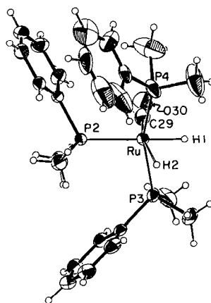
Fig. 3. ORTEP drawing of the molecular structure of 1a, cis , mer - \text{RuH}_2\text{CO}(\text{PMe}_2\text{Ph})_3 , showing atom labelling.
