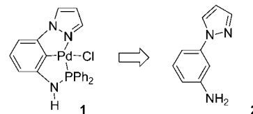
Figure 1. Existing PCN palladium complexes.
