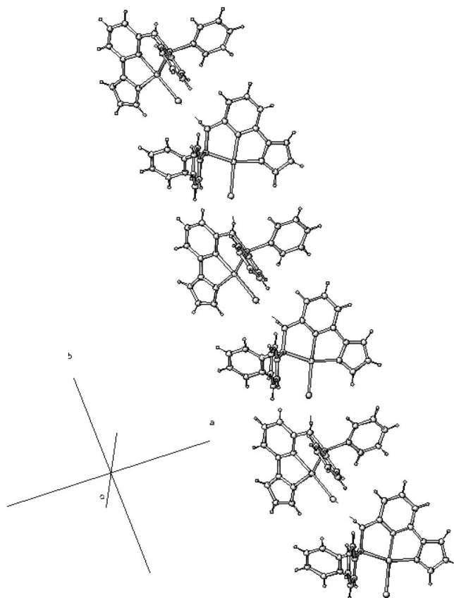
Figure 5. One-dimensional chain structure of complex 1 formed by C-H \cdots Cl hydrogen bonds.
