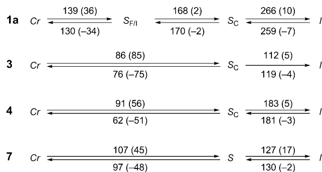
Fig. 1. Phase transitions of the compounds 1a , 3 , 4 , and 7 : onset temperatures [ ^{\circ} ] of the second heating curves and the first cooling curves. The numbers in parentheses indicate the enthalpies \Delta H in \text{kJmol}^{-1} ; \Delta H > 0 endothermic process, \Delta H < 0 exothermic phase transition. A rate of 10\text{ K min}^{-1} was used as temperature gradient.
