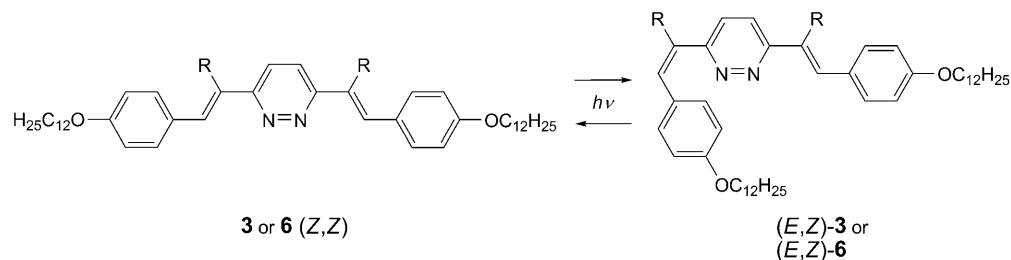
Scheme 4. Photoisomerization of (Z,Z)-Compounds 3 and 6 to Their (E,Z)-Isomers (E,Z)- 3 and 6 and (E,Z)- 6 , respectively
