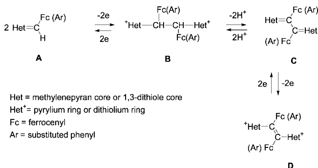
Scheme 1. Possible Reversible Steps in Aryl and Ferrocenyl Heterocyclic Series
