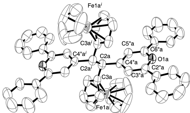
Figure 1. ORTEP drawing of molecule A in compound 2 with thermal ellipsoids at the 50% probability level. Labeling scheme, given here for molecule A with symmetries i : -x , 2-y , 1-z , is similar for molecule B with symmetries ii : 1-x , 1-y , -z .
