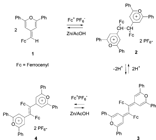
Scheme 2. Interconversions in Ferrocenylpyran Chemistry
